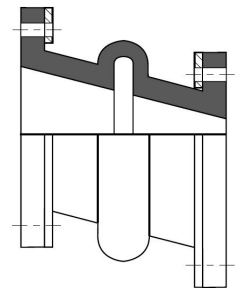
OFFSET
