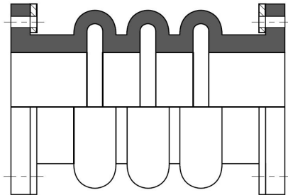
MULTIPLE ARCH
