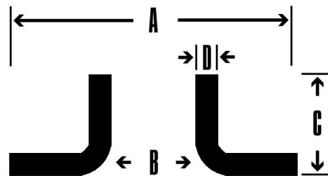
Flange (F)
