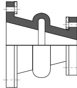
TAPERED
