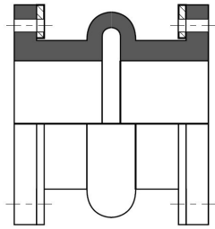
SINGLE ARCH
